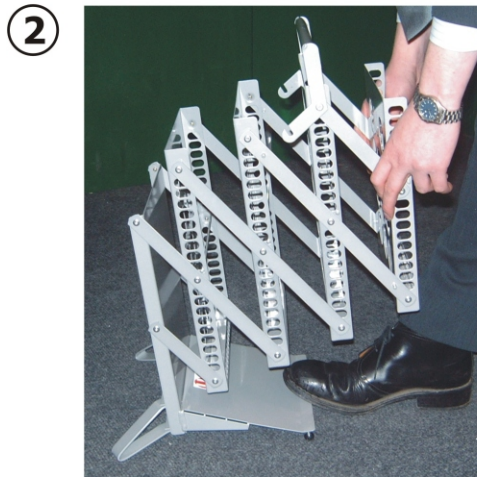
Release locking carry arm Whilst holding unit by sides of top tray, lift gently and place your foot lightly on the base to provide stability
